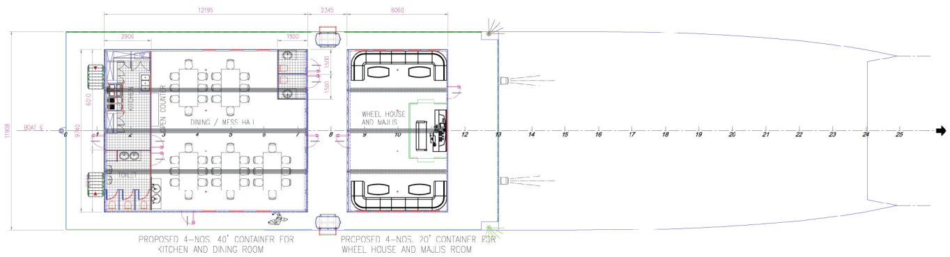
FIRST DECK LAYOUT PLAN
